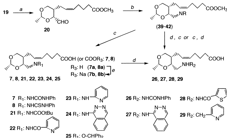
Scheme 2. (a) \text{CrO}_3 -2pyridine/ \text{CH}_2\text{Cl}_2 , rt; (b) \text{R}_1\text{NH}_2 or \text{R}_2\text{NH}_2 /AcOH/MeOH, rt; (c) 1 N NaOH/MeOH, rt; (d) \text{NaBH}_3\text{CN} /AcOH/MeOH, rt; (e) 1 N NaOH/MeOH, rt then treated at pH > 10.
