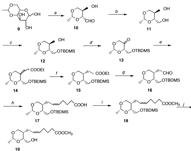
Scheme 1. (a) NaIO 4 /H 2 O, 5°C; (b) NaBH 4 /EtOH, 5°C; (c) TBDMSCl/imidazole/DMF, rt; (d) DMSO/DCC/TFA/pyridine/benzene, rt; (e) Ph 3 P=CHCOOEt/THF, rt; (f) 10%Pd-C/H 2 (3atm)/EtOH, rt then silica gel column; (g) DIBAL-H/toluene, –78°C; (h) NaH/DMSO, 75°C then (Ph 3 PC 4 H 9 COOH) + Br–/DMSO, rt; (i) CH 3 I/K 2 CO 3 /DMF, rt; (j) n -Bu 4 NF/THF, rt.
