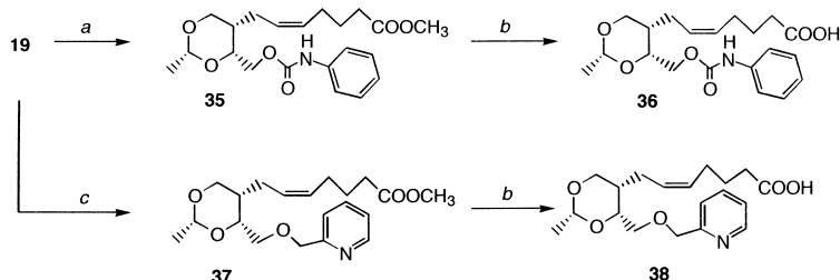
Scheme 4. (a) PhNCO/pyridine, rt; (b) 1 N NaOH/MeOH, rt; (c) 2-picolylchloride-HCl/NaH/DMF, rt.
