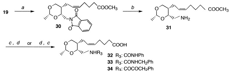
Scheme 3. (a) TsCl/pyridine, rt then potassium phthalimide/DMSO, 100°C; (b) \text{H}_2\text{NNH}_2 \cdot \text{H}_2\text{O} /EtOH, rt; (c) PhNCO/pyridine, rt or PhCH 2 NCO/pyridine, rt or PhCH 2 COCOOH/DCC/EtOAc, rt; (d) 1 N NaOH/MeOH, rt.
